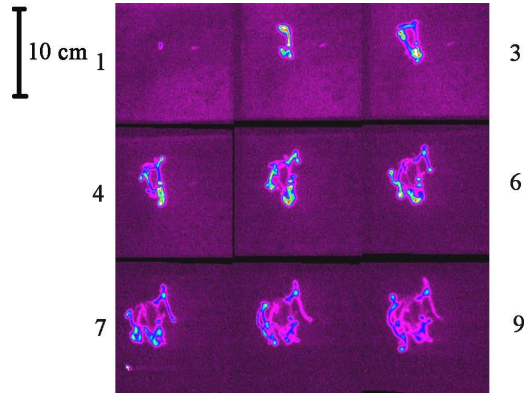
Fig. 11. Developed streamer MW discharge: p = 150 Torr, E_0 = 2800 V/cm, t_{\text{exp}} = 0.5 \mu\text{s} , t_p = 2 \mu\text{s}
